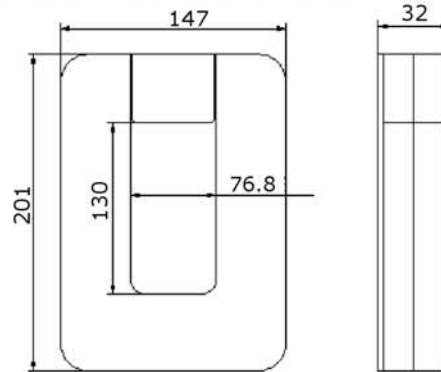
Dimensions: (unit:mm)
