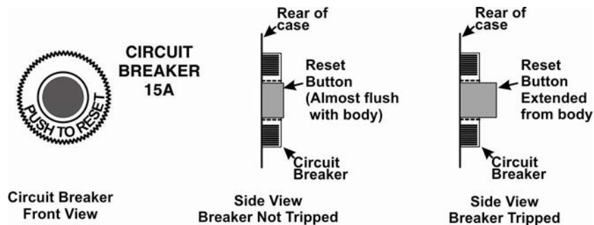
Figure 137- Circuit Breaker Protection
