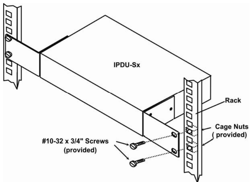
Figure 10- Secure IPDU-Sx to rack
