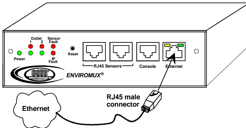
Figure 2- Connect IPDU-S2 to the Ethernet
