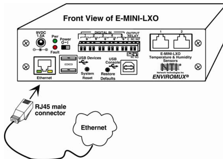
Figure 8- Connect E-MINI-LXO to the Ethernet
