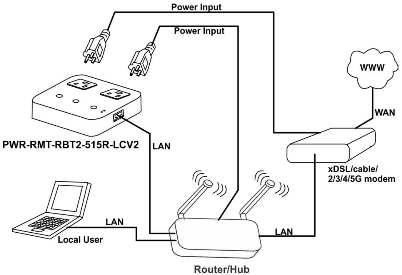
PWR-RMT-RBT2-515R-LCV2 setup to perform auto reset of router and modem
